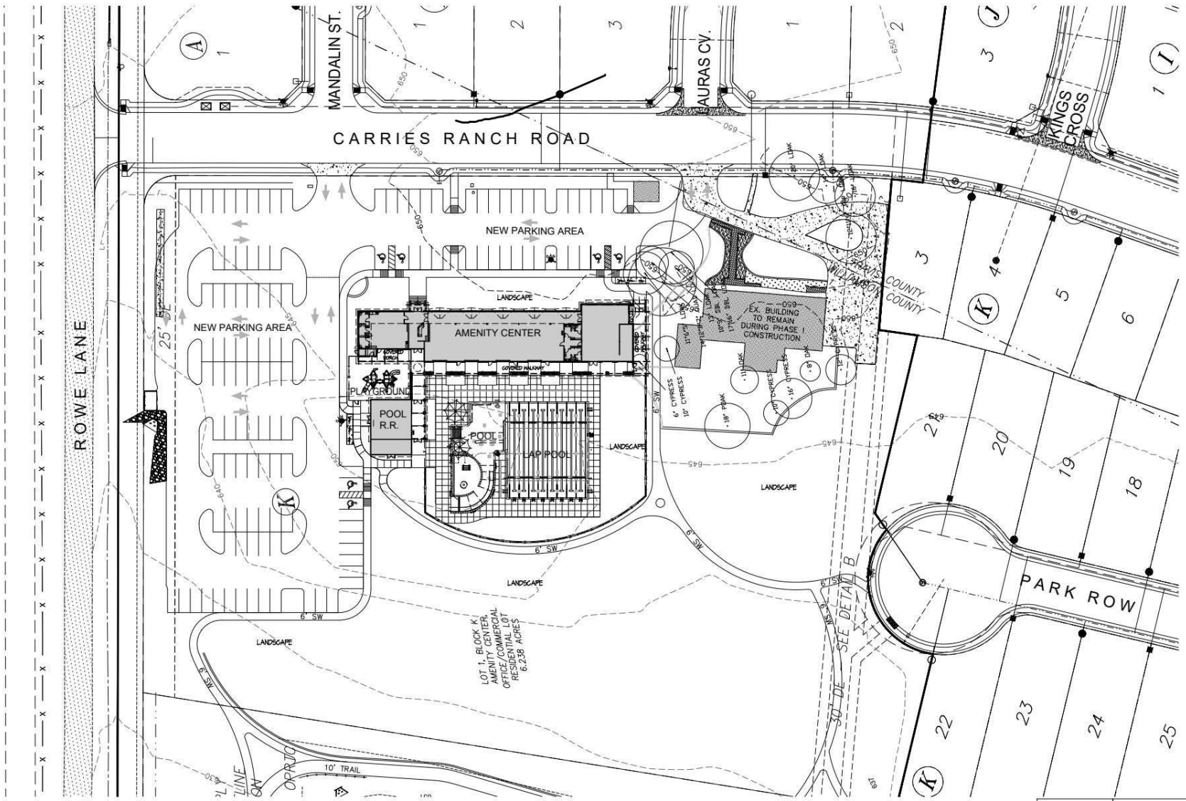
01 OVERALL SITE PLAN Scale: 1" = 30'-0"
